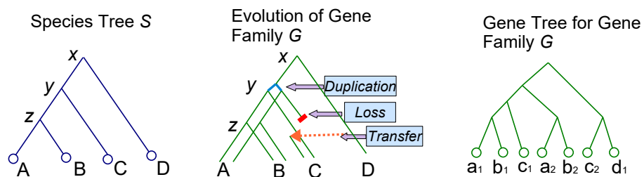
Figure 1: Gene family evolution. This figure shows a possible evolutionary history of some gene family G (middle) that evolves along the branches/lineages of the depicted species tree S (left). The gene family G starts as a single gene in the ancestral species represented by the root of S and evolves along the branches of the species tree where it is affected by duplication, transfer, and loss events, in addition to speciation. The tree on the right represents the gene tree topology for G that would result if one were to use all extant homologous gene sequences from gene family G (i.e., all gene from G present in species A , B , C , and D ) and reconstruct a gene tree on those gene sequences. The leaves labeled with lower-case letters in the gene tree represent genes sampled from the corresponding upper-case species, e.g., genes a_1 and a_2 represent the two genes from G present in species A .
