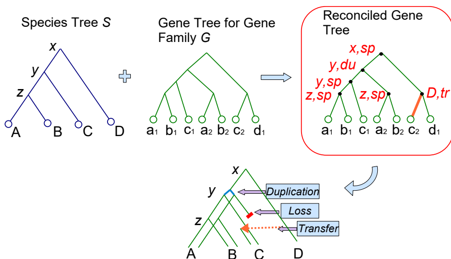
Figure 2: DTL reconciliation output. The two trees on the left are the rooted species tree and rooted gene tree being reconciled. The tree on the right, within the red box, depicts the result of applying DTL reconciliation to the trees on the left. Specifically, DTL reconciliation labels each internal node of the gene tree with a mapping to a node of the species tree and an event type ( sp , du , and tr for speciation, duplication, and transfer, respectively). The reconciliation also specifies the edges of the gene tree, marked in bold orange, that represent transfer edges. These events and mappings show how the gene tree may have evolved inside the species tree. The reconciliation (i.e., labeled gene tree) shown in this figure implies that gene family G evolved inside the species tree as shown at the bottom.
